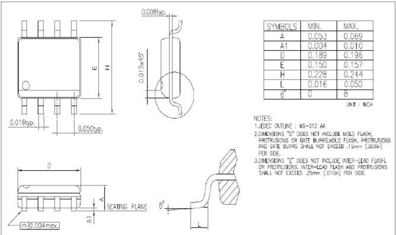
8-Pin 150mil SOP Package
