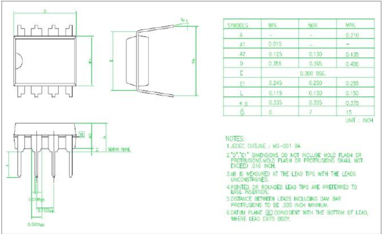
8-Pin 300mil P-DIP Package
